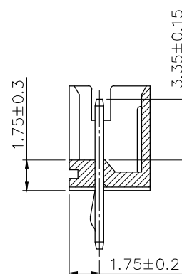
SECTION M-M
