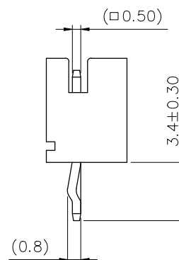
SECTION M-M
